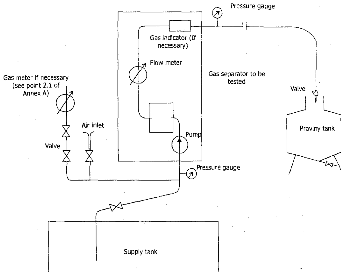
FIGURE-6 TESTING FACILITY FOR GAS SEPARATORS IN FUEL DISPENSERS
